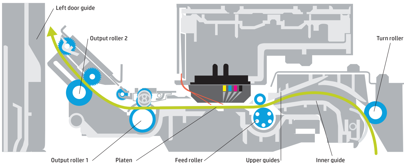
Figure 9: Cross-section of the paper transport
