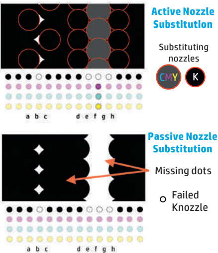
Figure 7: Schematic: nozzle substitution
