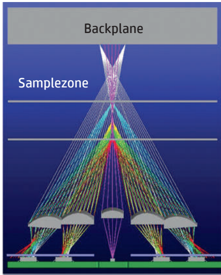
Figure 6: Schematic of Backscatter Drop Detection
